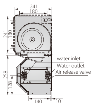
2-pipe duct
